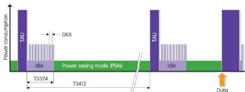
Fig. 5 power consumption diagram
