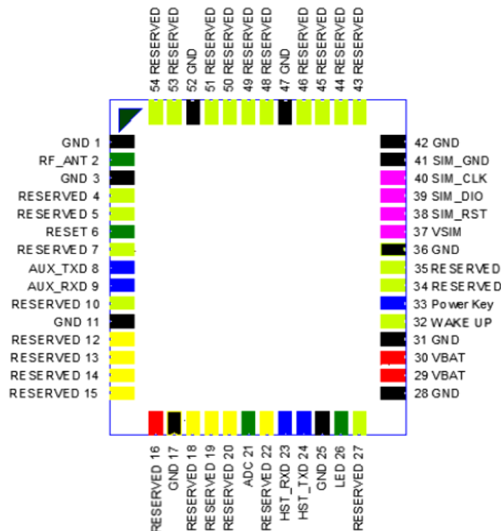
Fig. 1 Diagram of pin distribution
